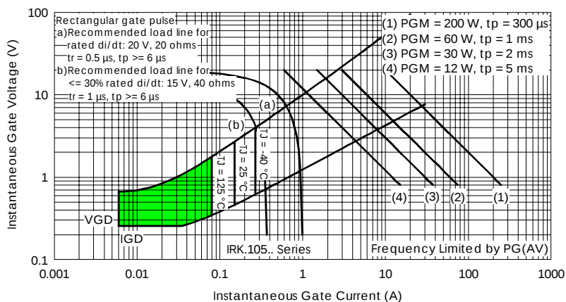
Fig. 13- Gate Characteristics
