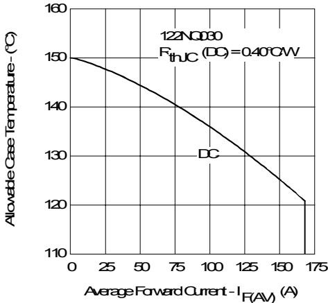
Fig. 5-Maximum Allowable Case Temperature Vs. Average Forward Current
