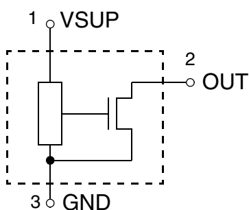
Fig. 4–3: Pin configuration
