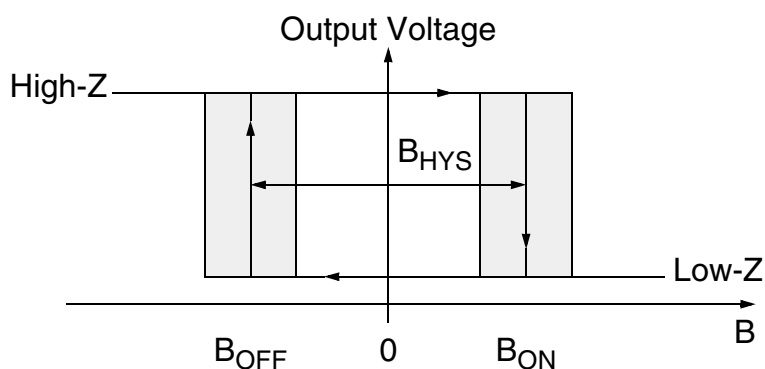
Fig. 4–5: Definition of magnetic switching points for the HAL 1502
