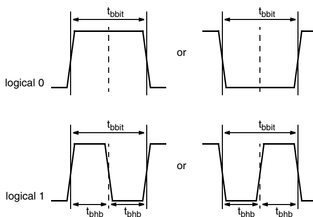
Fig. 12–1: Definition of logical 0 and 1 bit
