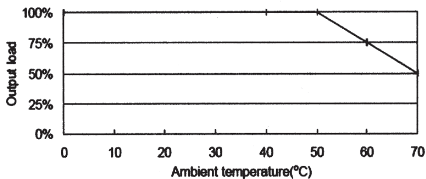
ZPS100-12 -15 -18 -24 -28 DERATING CURVE
