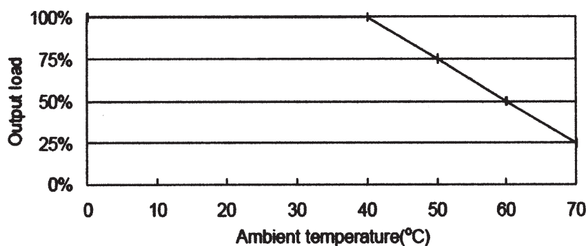
ZPS100-3R3 -5 -9 -48 DERATING CURVE
