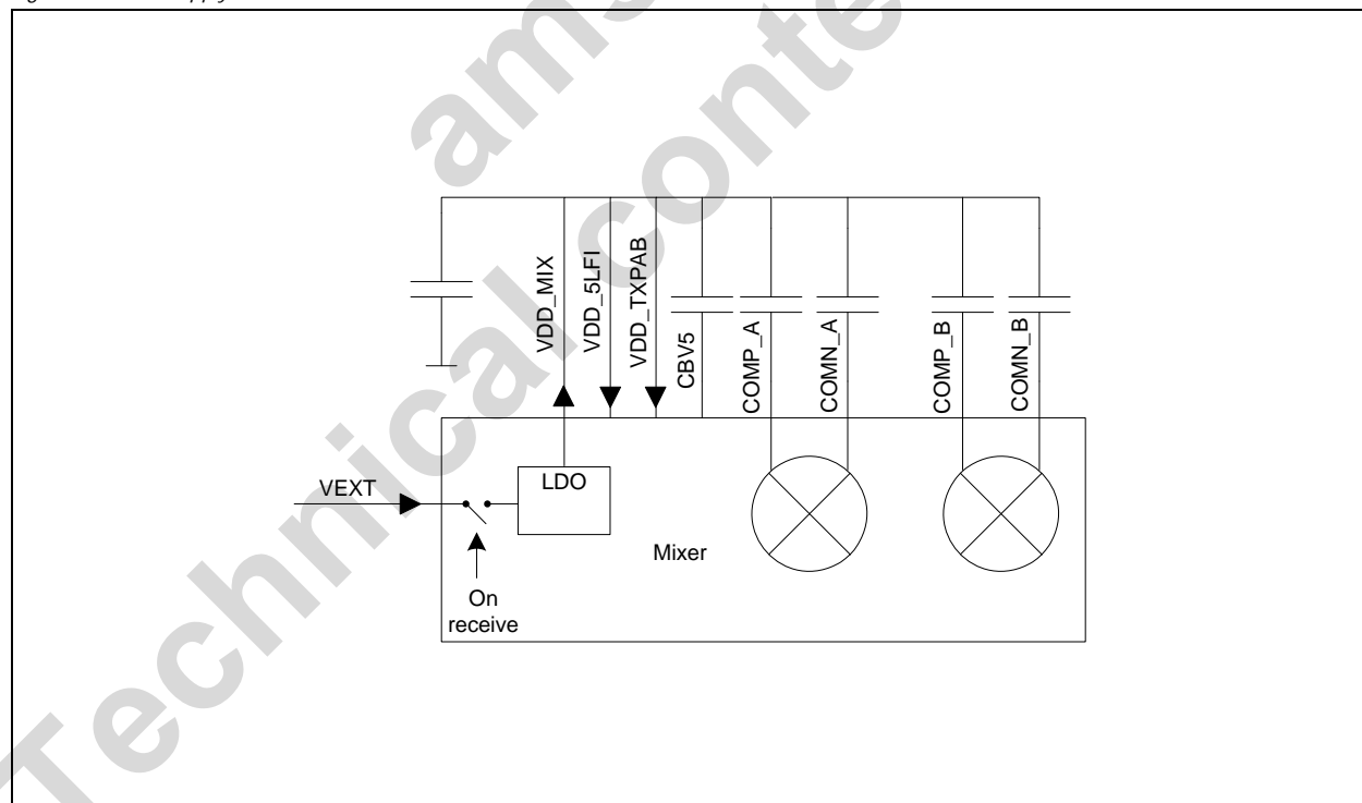
Figure 3. Mixer Supply
