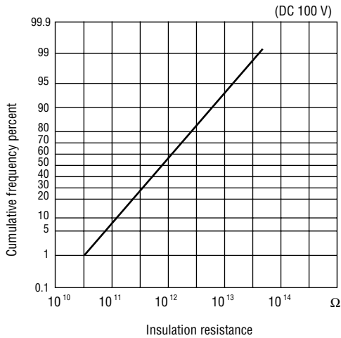
(4) Insulation resistance
