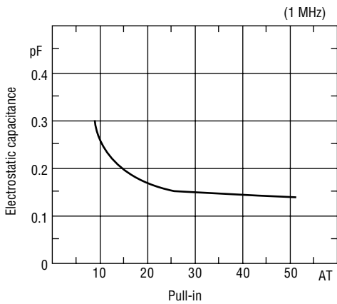
(5) Electrostatic capacitance
