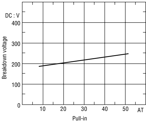
(3) Breakdown voltage
