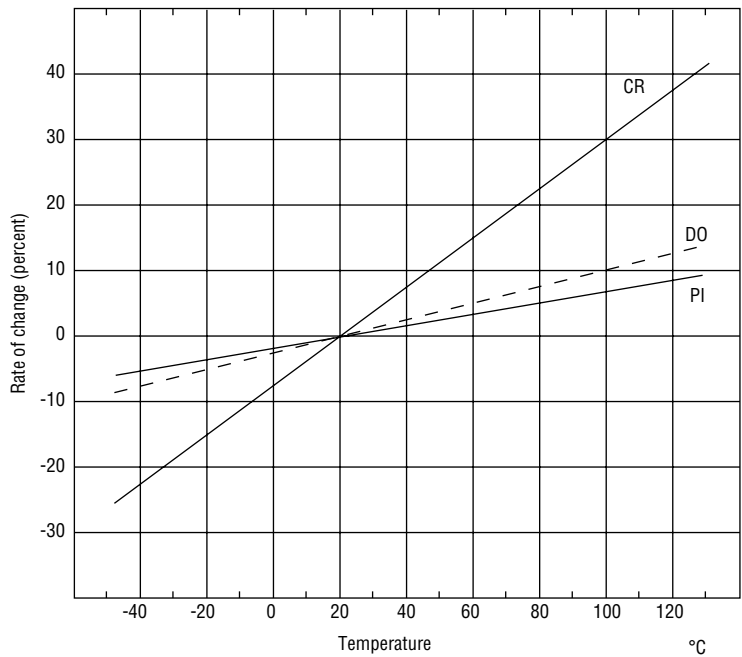
(1) Temperature characteristics
