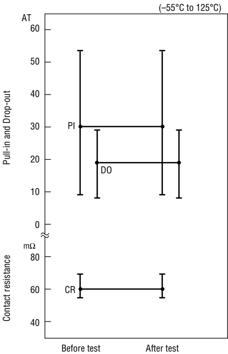
(2) Temperature cycle
