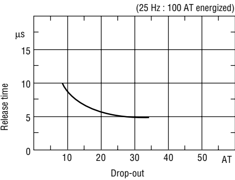
(3) Release time
