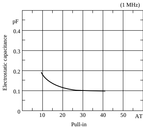
(5) Electrostatic capacitance
