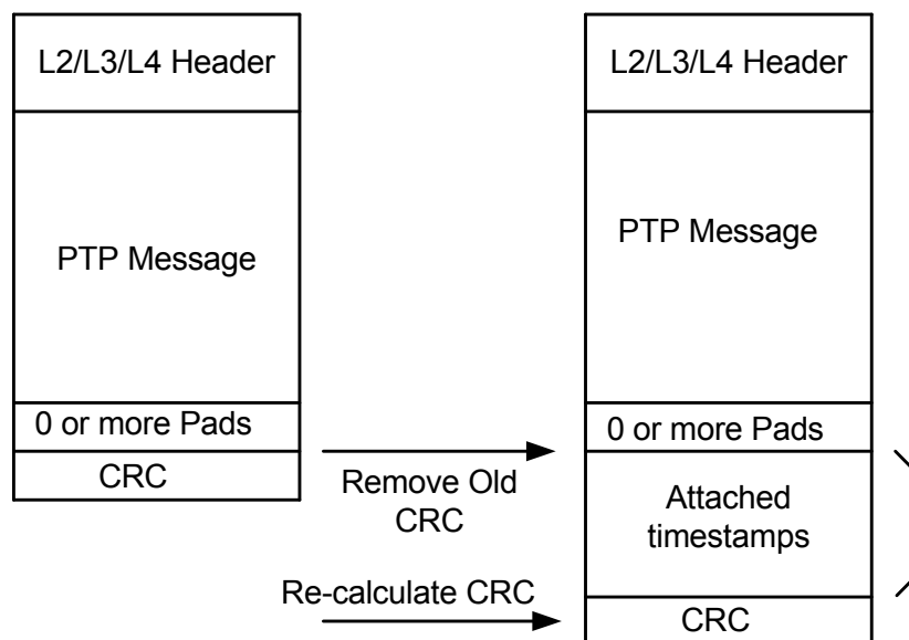
Figure 2-14. PTP Timestamp.
