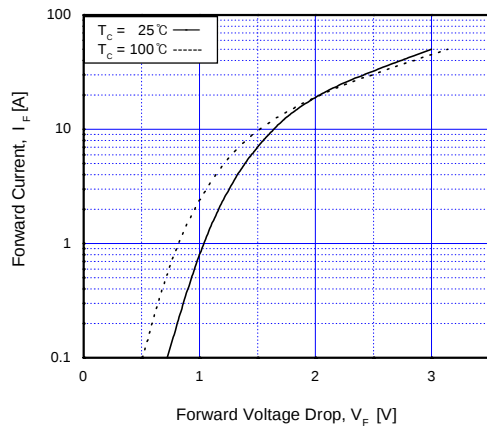
Fig 18. Forward Characteristics
