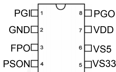
Figure 4. Pin Configuration
