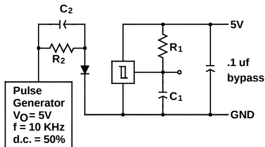
Fig. 8 Switching Speed Test Circuit
