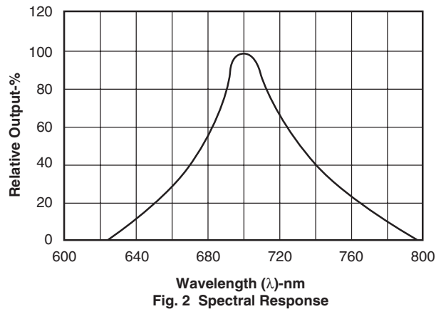
Fig. 2 Spectral Response
