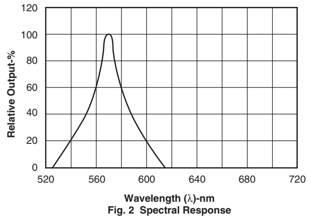
Fig. 2 Spectral Response
