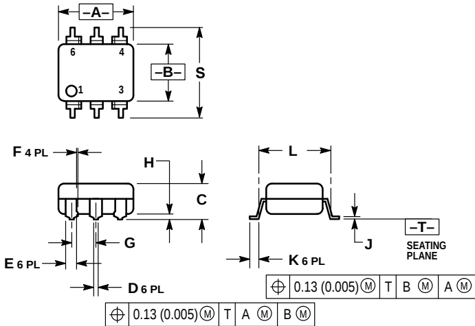
SURFACE MOUNT
