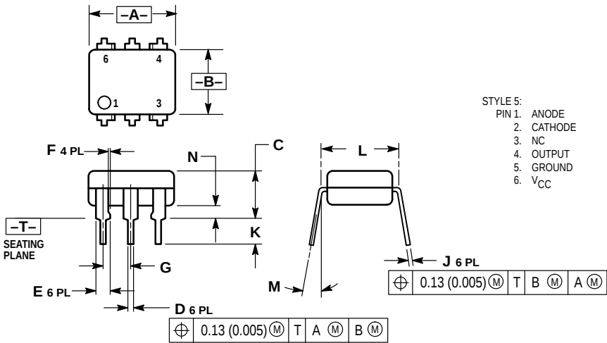
THRU HOLE
