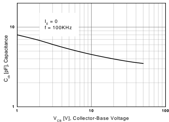
Figure 5. Collector-Base Capacitance
