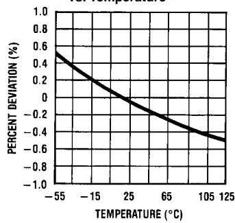
Typical 1 ms Pulse Width Variation vs. Temperature
