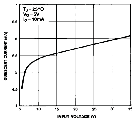
Figure 4. Quiescent Current
