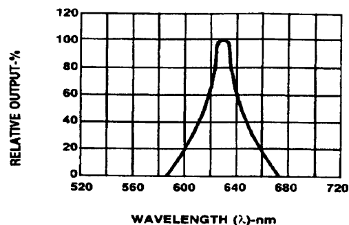
Fig.2 SPECTRAL RESPONSE
