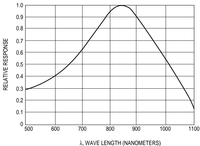
Figure 5. Spectral Response
