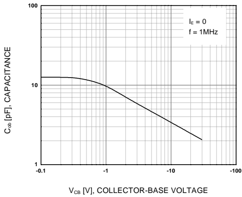
Figure 3. Output Capacitance
