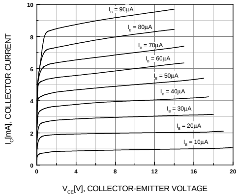
Figure 1. Static Charateristics
