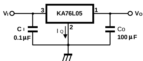
Figure 1. Application Circuit
