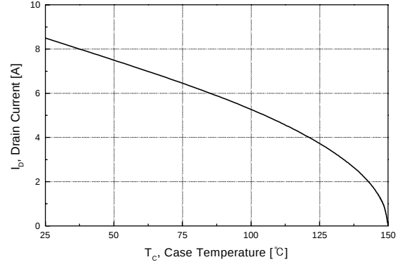
Figure 10. Max. Drain Current vs. Case Temperature
