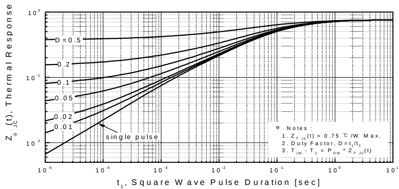
Figure 11. Thermal Response
