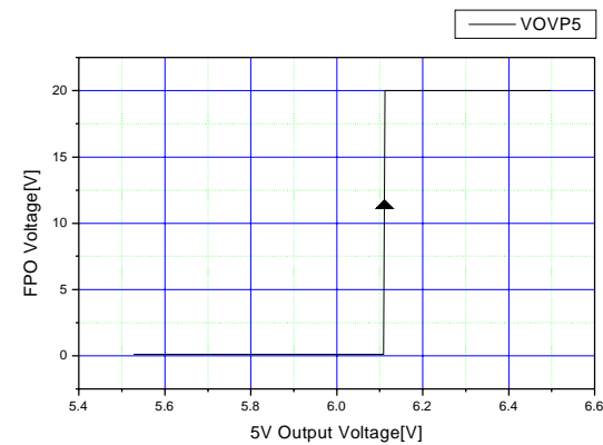
Figure 3. Over Voltage Protection for +5V
