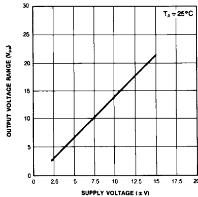
Figure 3. Output Swing
