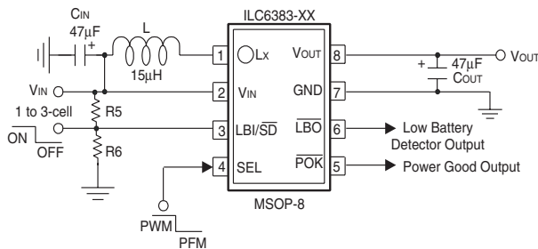
Figure 1. ILC6383CIR-XX
