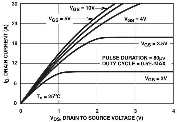
FIGURE 8. SATURATION CHARACTERISTICS
