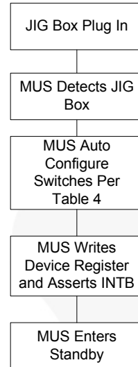
Figure 4. JIG Box Detection Flow
