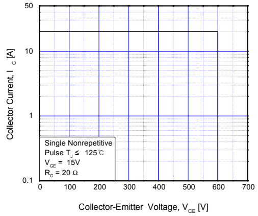
Figure 16. RBSOA Characteristics
