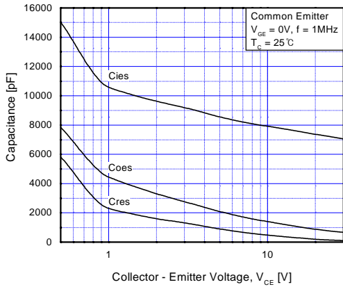
Fig 7. Capacitance Characteristics
