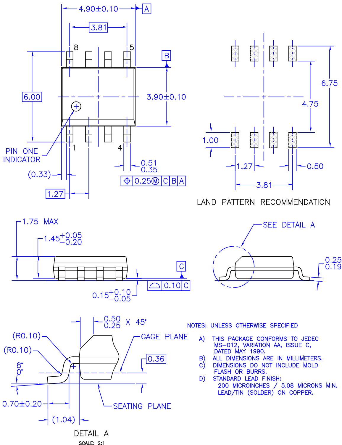
Figure 17. Molded Package, Small Outline, 0.15 Wide, 8-Lead (M8)
