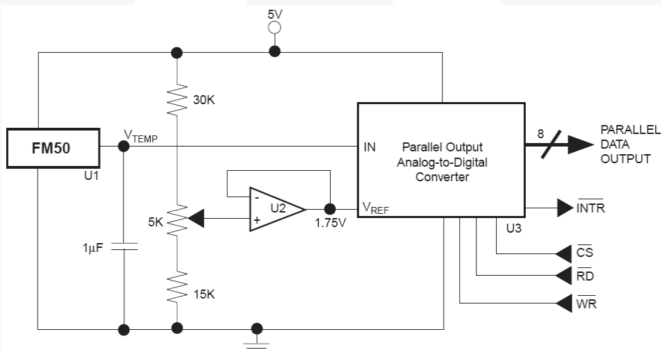
Figure 8. Parallel Output Temperature to Digital Converter (Full Scale = +125°C)
