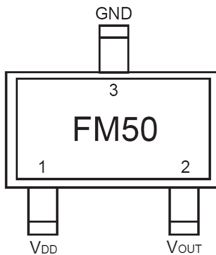
Figure 2. Pin Configuration
