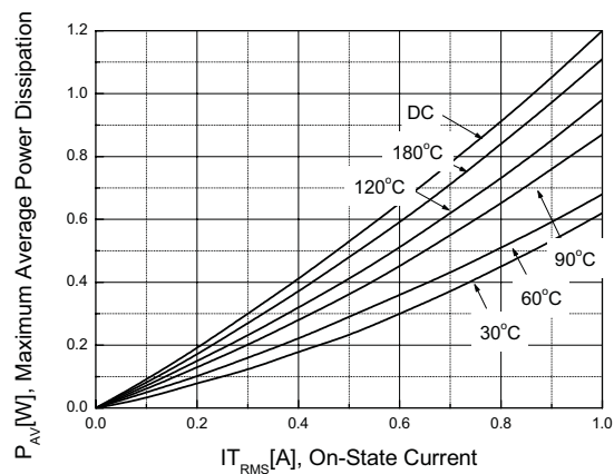
Figure 2. Power Dissipation
