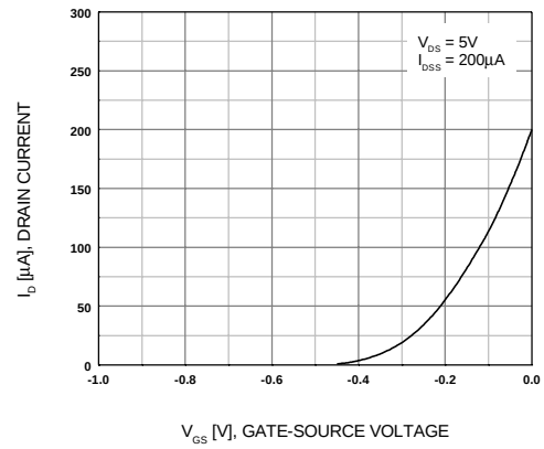
Figure 2. Transfer Characteristic
