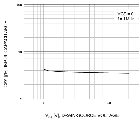
Figure 5. Input Capacitance
