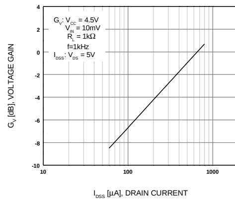
Figure 14. Voltage Gain
