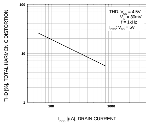
Figure 11. Total Harmonic Distortion vs. I_{DSS}
