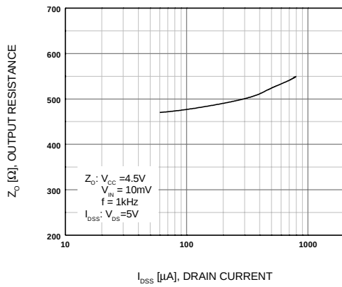
Figure 9. Output Resistance
