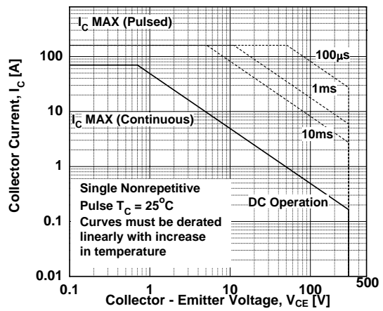
Figure 10. SOA Characteristics
