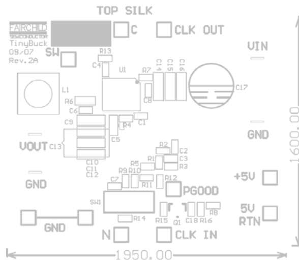
Figure 3. Assembly Diagram
