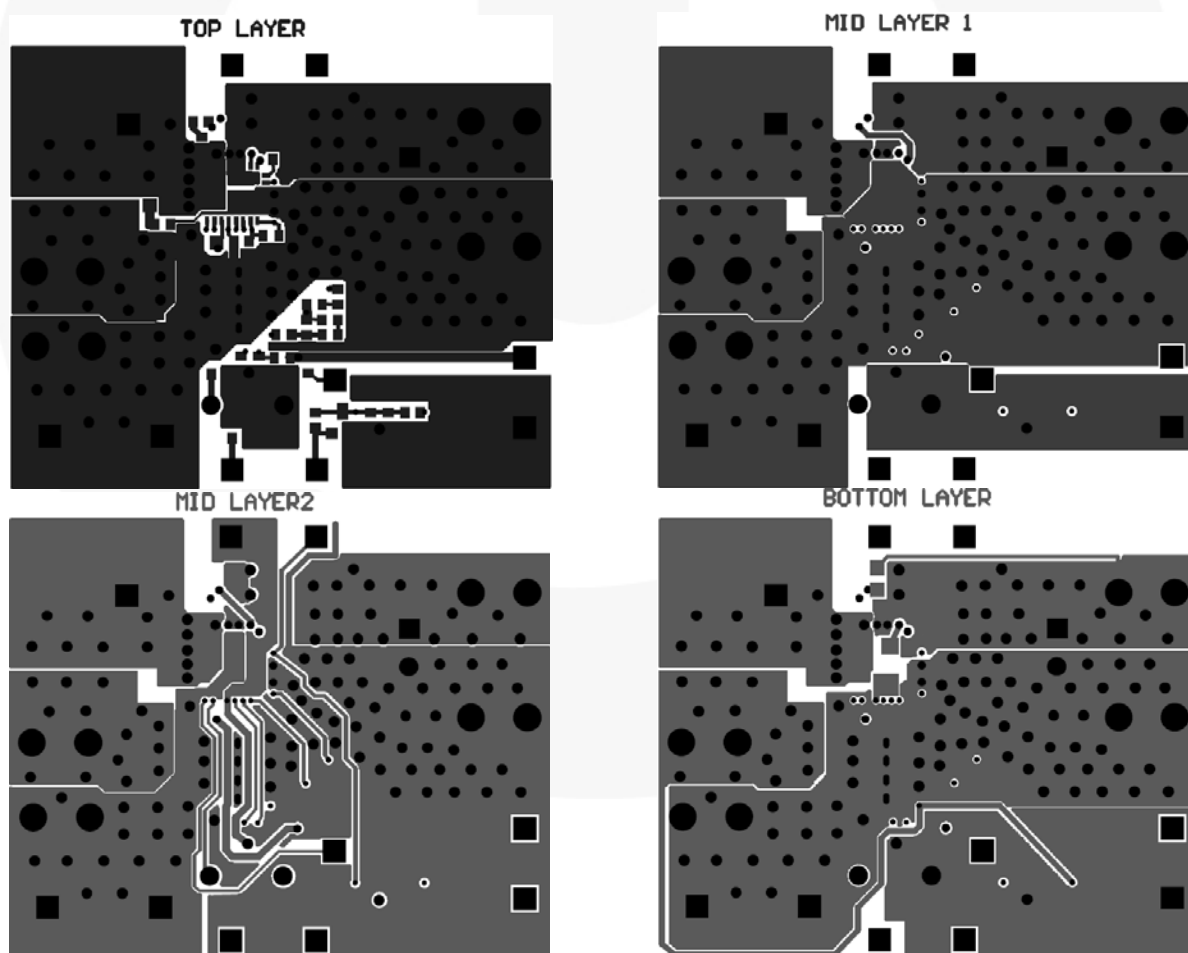
Figure 4. PCB Layout
