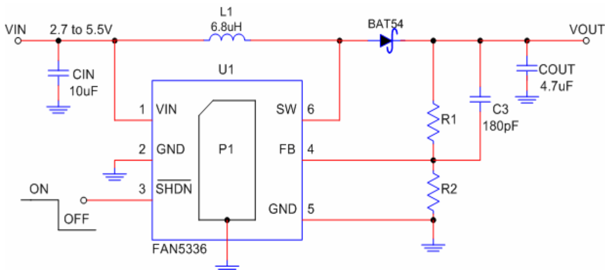
Figure 2: Schematic Diagram
