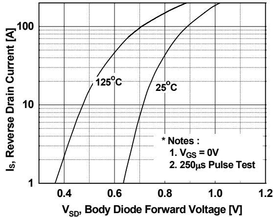
Figure 5. Body Diode Forward Voltage Variation vs. Source Current and Temperature
