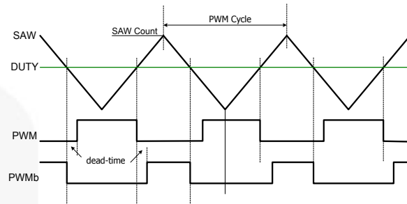
Figure 17. PWM Output
