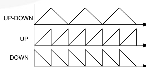
Figure 16. SAW Output Mode
