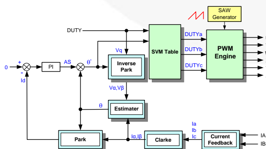
Figure 13. Speed Integral Block Diagram
