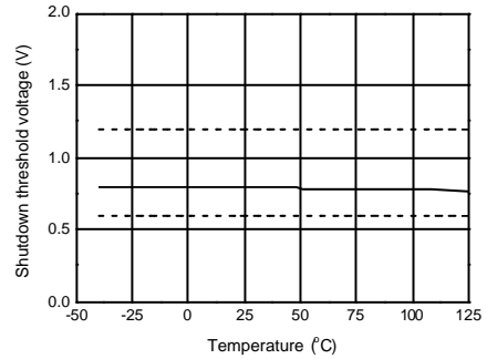
Figure 29. Shutdown Threshold of vs Temperature
