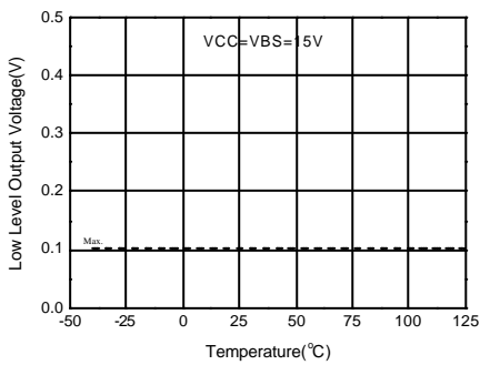
Figure 18a. Low Level Output of HO vs Temperature
