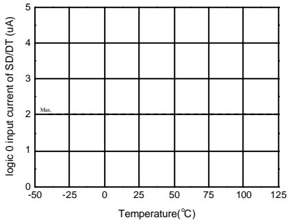
Figure 28. Logic 0 Input Current of SD/DT vs Temperature
