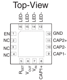
FAN5607 4x4mm 16-Lead MLP
