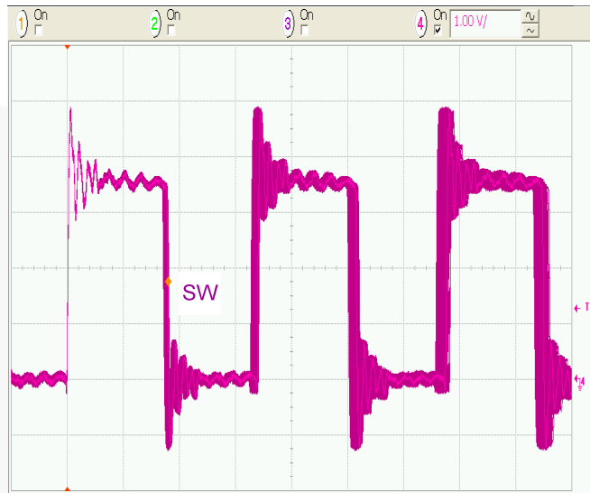
Figure 39. SW-Node Jitter (Infinite Persistence), I_{LOAD} = 200mA , 50ns/div .
