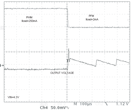
Figure 10. Load Transient Response
