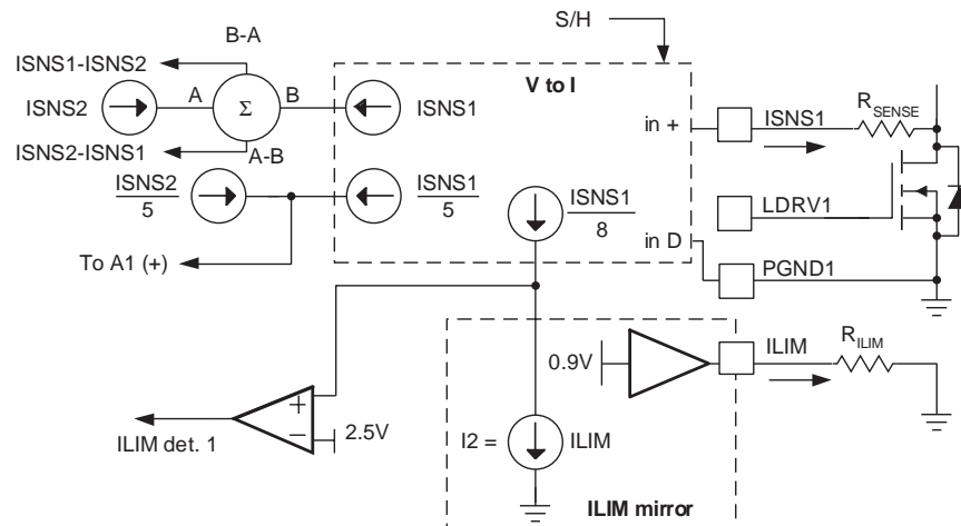
Figure 6. Current Limit and Active Droop Circuits
