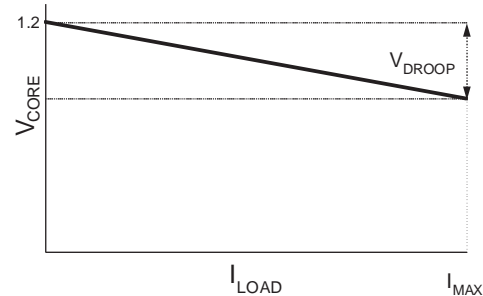
Figure 5. Active Droop
