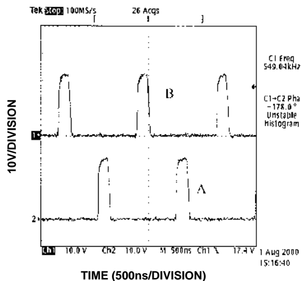
HIGH-SIDE GATE DRIVES, NORMAL OPERATION
