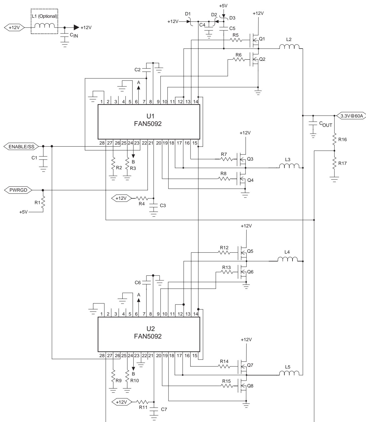
Figure 1. Four-Phase Application Circuit
