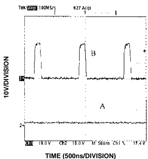
HIGH-SIDE GATE DRIVES, E*-MODE
