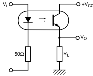
Fig. 2 Switching Circuit
