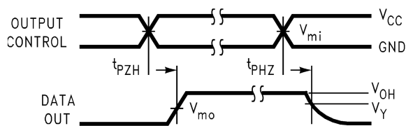
FIGURE 7. 3-STATE Output Enable and Disable Times for Low Voltage Logic
