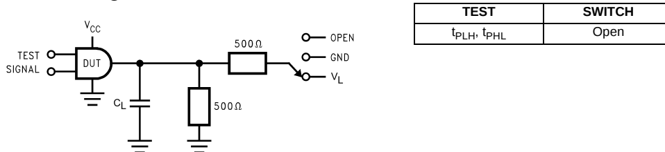
FIGURE 1. AC Test Circuit
