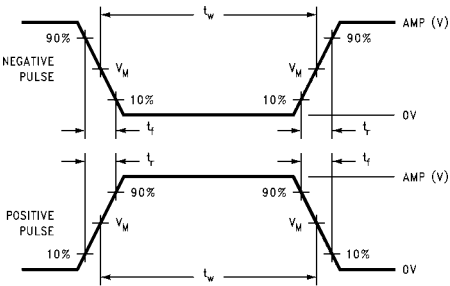
FIGURE 2. V_M = 1.5\text{V} Input Pulse Requirements
